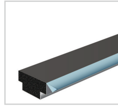
Flexible Spacer with stepped profile for application of PIB. (Auto Reels - 6.3mm Profile Height)
